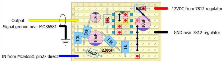
Complete through view (transparent pcb)
