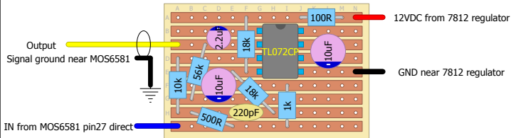
Component view
